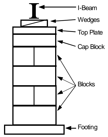
Double Block Pier Construction
